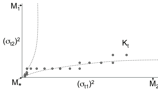
FIG. 1. 2-dimensional projection of \mathcal{K} for the ranking and selection problem. The dimensions pictured are the posterior variances \sigma_{i_1}^2 and \sigma_{i_2}^2 . The vertical axis is M_1 , where \sigma_{i_1}^2 = 0 and the first alternative's sampling mean is known. Similarly, the horizontal axis is M_2 . Their intersection is M_* . Dashed lines give open regions around M_1 and M_2 in which stuck alternatives are not measured, and the dots K_t are a sequence of knowledge states converging to M_* .
